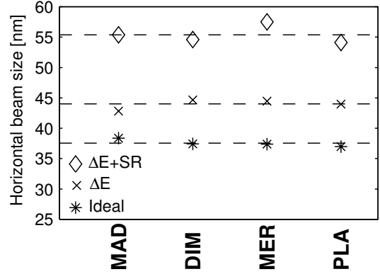
Figure 5: Comparison of the horizontal beam sizes calculated with a Gaussian fit. On the x axis there are the four considered codes and on the y axis the horizontal beam size. The points are the average of the data of Table 4. On this scale the error bars due to statistical fluctuations are negligible and have been omitted.
