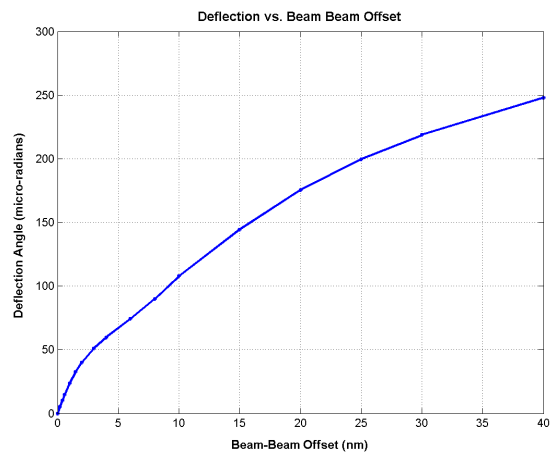
Figure 2. Beam-Beam deflection vs. beam offset for nominal NLC interaction point parameters[4].
